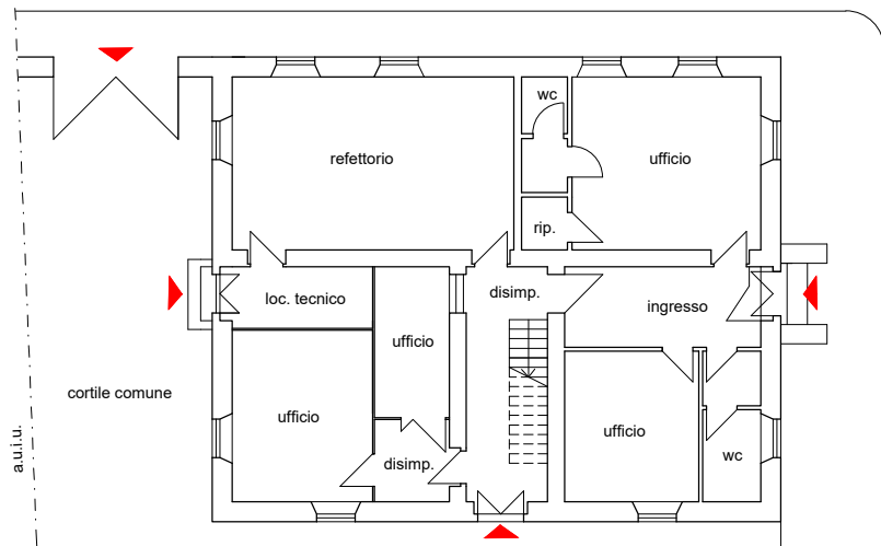
Piano Terra (fabbr. A) h=3.55 m
